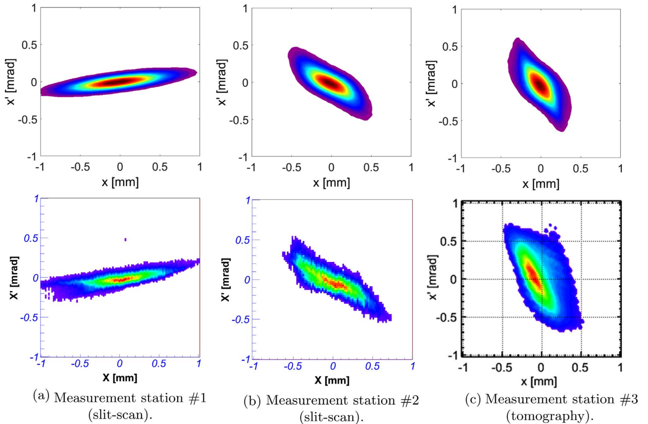
Fig. 3. Simulated (top) and measured (bottom) horizontal trace-space distributions at the three measurement stations. The colour code represents normalized charge density (maximum is red, minimum is violet). (For interpretation of the references to colour in this figure caption, the reader is referred to the web version of this paper.)
