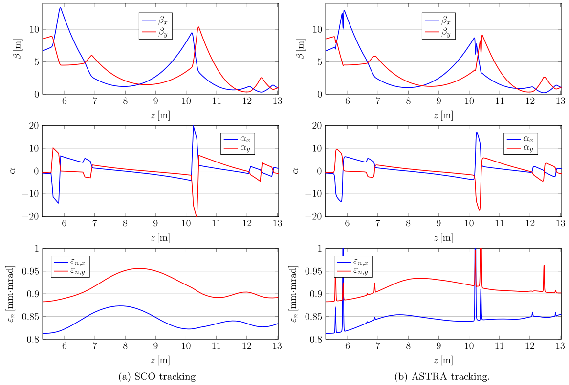
Fig. 2. Evolution of the \beta -function (top), \alpha -function (middle) and normalized emittance (bottom) of the horizontal (blue line) and the vertical plane (red line) along the matching lattice, according to SCO (left) and ASTRA (right). (For interpretation of the references to colour in this figure caption, the reader is referred to the web version of this paper.)
