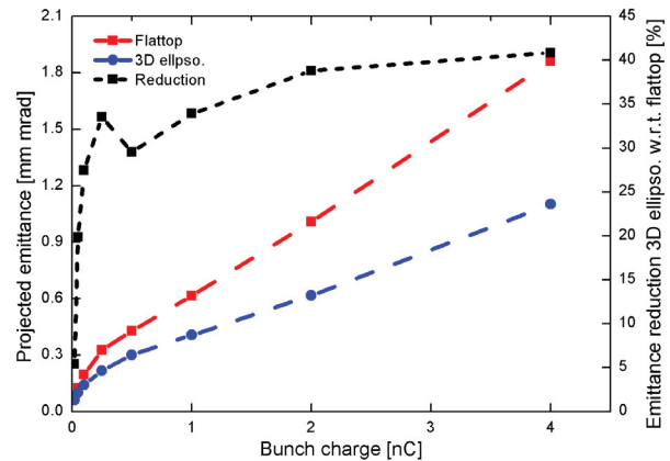
Figure 5: Electron beam transverse emittance as a function of bunch charge for flattop and ellipsoidal laser profiles at EMSY1 in the left axis, and in the right axis the emittance gain from ellipsoidal beams with respect to flattop ones.
