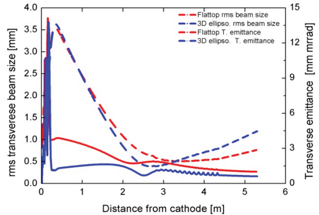
Figure 2: Transverse projected emittance and rms beam size for 2 nC bunch charge along the beamline up to EMSY1.
