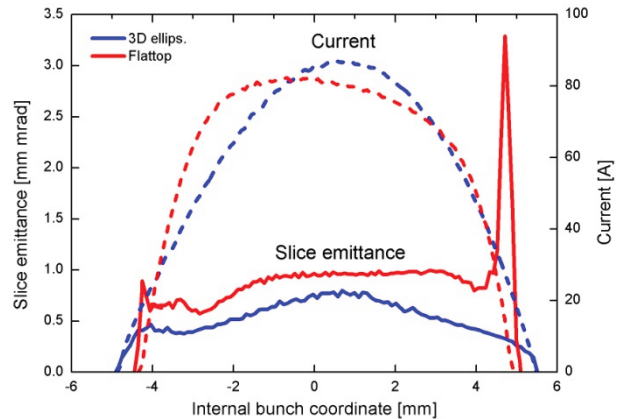
Figure 3: Beam current and slice transverse emittance distribution within the bunch for 2 nC bunch charge at EMSY1.
