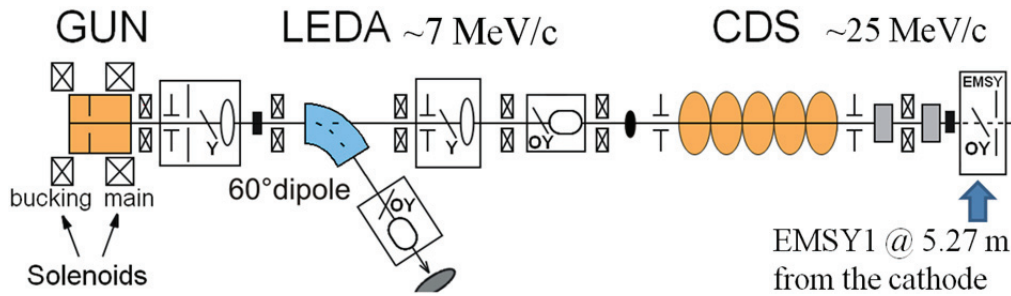
Figure 1: Schematic layout of the current PITZ beamline used in ASTRA simulations up to EMSY1.
