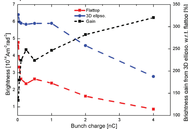
Figure 6: Brightness of the electron beam as a function of bunch charge for flattop and ellipsoidal laser profiles in the left axis, and in the right axis the brightness gain from ellipsoidal beams with respect to flattop ones.
