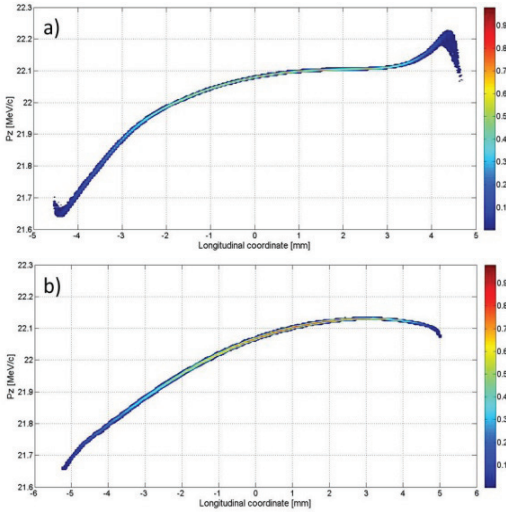
Figure 4: Electron beam longitudinal phase space for 2 nC bunch charge generated from (a) flattop and (b) ellipsoidal cathode laser pulses.
