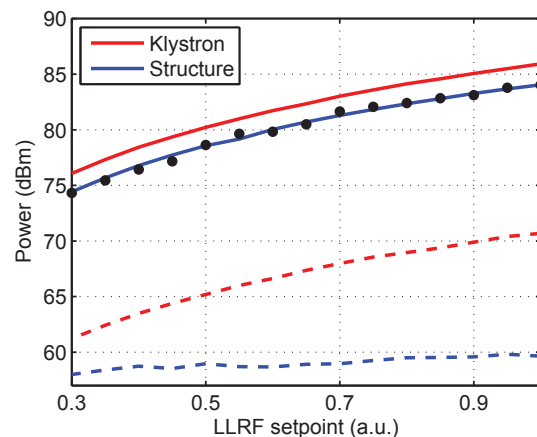
Figure 3: Forward (full lines) and reflected (dashed lines) power readings from the directional couplers at the klystron and deflecting structure. The black dots are estimations of the power in the structure based on the measured electron beam deflection.
