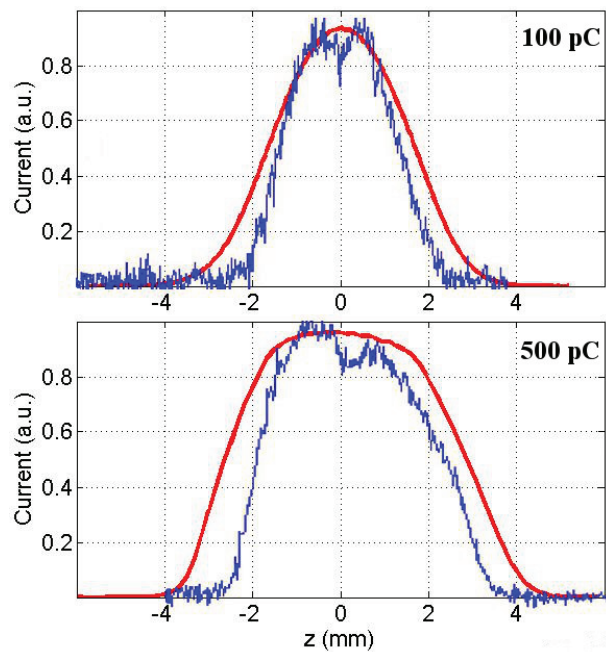
Figure 5: Longitudinal profiles of 100 pC (top) and 500 pC (bottom) bunches after the TDS. The smooth red curves are ASTRA simulations assuming a 11.5 ps (FWHM) long Gaussian photocathode laser pulse, the blue curves are TDS measurements.
