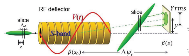
Figure 1: TDS principle: Depending on their longitudinal position, electrons are deflected by transverse RF fields and observed on a screen several meters downstream [4].
