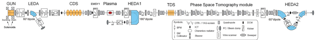
Figure 2: Current layout of the PITZ beamline (PITZ 3.0). Electron bunches which are streaked vertically by the TDS can be monitored on several YAG and OTR screens in the tomography module. Alternatively, their full longitudinal phasespace can be analyzed in the high energy dispersive arm HEDA2, 7.3 m downstream the TDS. During the measurements presented in this paper, the plasma cell was replaced by an empty beam tube.
