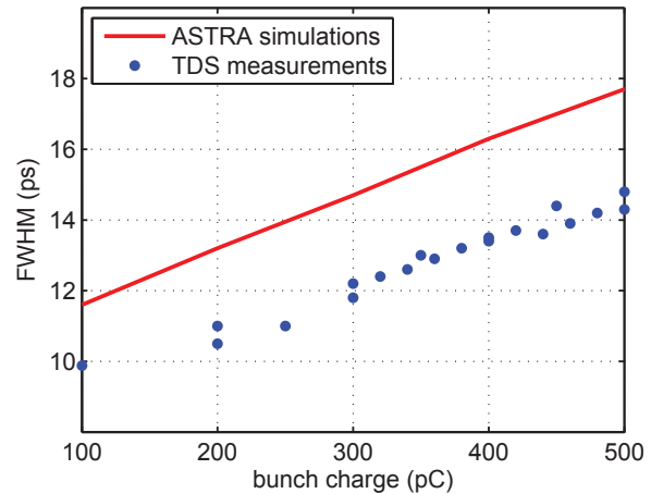
Figure 4: FWHM bunch lengths, measured and simulated, for bunch charges between 100 and 500 pC. The booster phase was tuned for maximum mean momentum gain.
