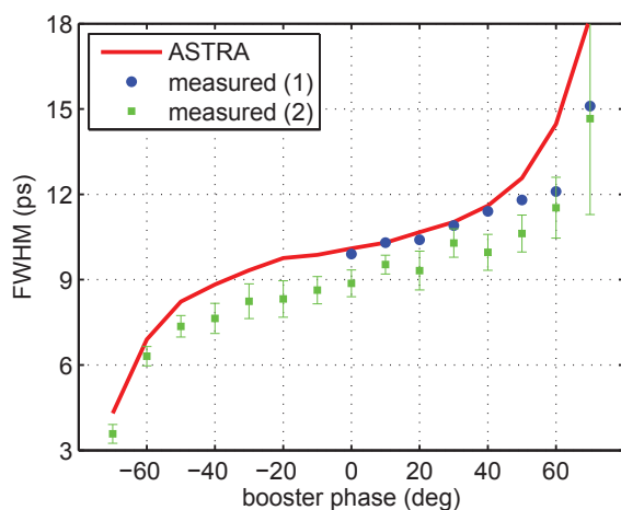
Figure 6: FWHM bunch length versus booster phase for a bunch charge of 100 pC, measured with the TDS (two data sets) and simulated (red line) using the measured transverse laser profile from the first data set (blue dots) as input.
