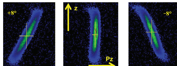
Figure 7: First low-resolution images of the full longitudinal phase space, viewed on a YAG screen after the first HEDA2 dipole magnet. The left and right pictures were taken at +8 and -8 degree booster phase with respect to the maximum mean momentum gain phase, respectively.
