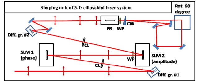
Figure 2: Setup of the 3-D pulse shaper; SLM – spatial light modulator, Diff. gr. – diffraction grating, WP – half-wave plate, CL – cylindrical lens, FR – Faraday rotator, CW – calcite wedge, Rot. 90 degree – laser beam rotator 90°.
