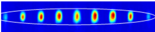
Figure 4: Scanning cross-correlator measurements of spatial and temporal shaped laser pulses (before harmonics generation), \sim 1.7 ps time steps between images.
