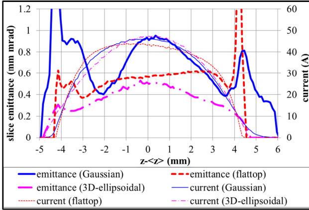
Figure 1: Beam dynamics simulation of electron bunches for photo cathode laser pulses with flat-top, Gaussian and 3-D ellipsoidal temporal profiles; normalized transverse slice emittance \epsilon_{\text{slice}} distribution along the electron bunch.
