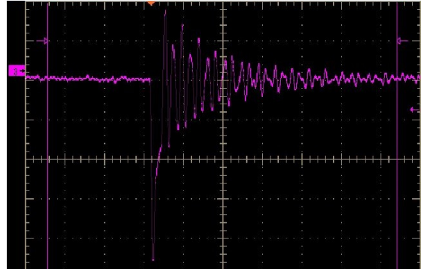
Figure 5: Charge measurement (Faraday cup) of electron bunch generated by new laser system; bunch charge about 50 pC.
