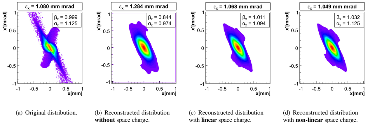
Figure 2: Horizontal plane of the original and reconstructed phase-space distributions with their corresponding normalized emittance values and Twiss parameters.
