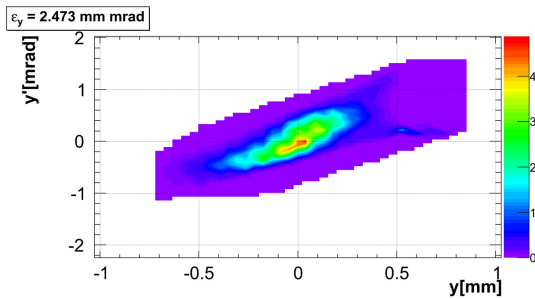
(a) Result without space-charge consideration.
