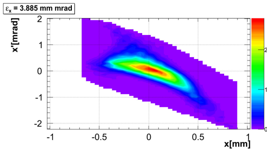
(a) Result without space-charge consideration.
