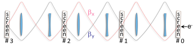
Figure 1: Schematic layout of the tomography section at PITZ. The beam propagates from right to left through six focusing and defocusing quadrupoles represented as lenses. Four intercepting screens capture projections of each transverse phase plane ideally at equidistant phase advance values as indicated by the plotted \beta -functions.
