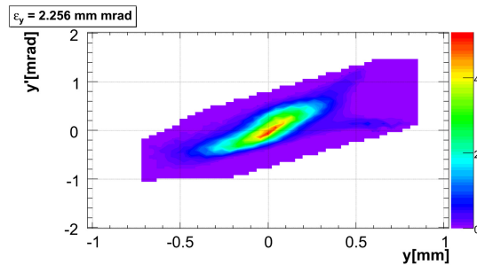
(b) Result with linear space-charge consideration.
