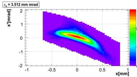
(b) Result with linear space-charge consideration.
