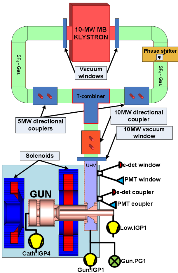
Figure 1: Gun conditioning setup: gun and RF system overview, vacuum pumps and IL detector locations.
