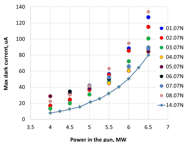
Figure 10: Maximum dark current dependence on the peak power in gun on different days.
