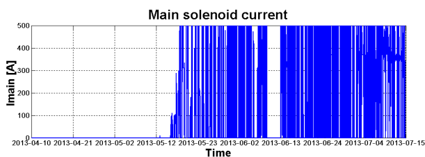
Figure 7: Main solenoid current history during gun conditioning.
