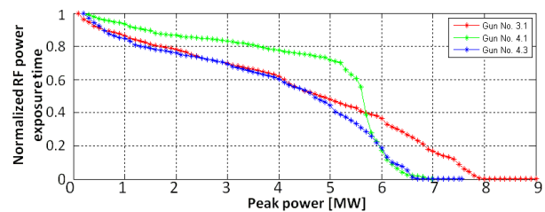
Figure 5: Comparison of the normalized RF exposure time for Gun 3.1, Gun 4.1 and Gun 4.3.
