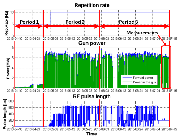
Figure 2: History of the Gun 4.3 conditioning. Top – Repetition rate, middle – forward power and power in the gun, bottom – RF pulse length.
