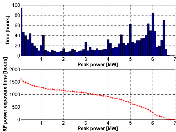
Figure 3: Gun 4.3 run statistics for peak power in the gun cavity.
