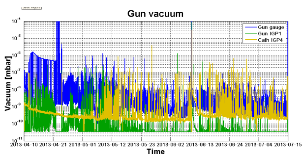
Figure 8: Vacuum activity during gun conditioning.
