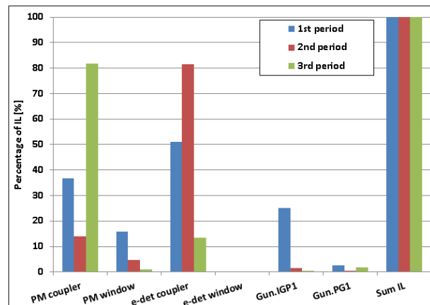
Figure 6: Percentage of interlocks for different periods of the gun conditioning.
