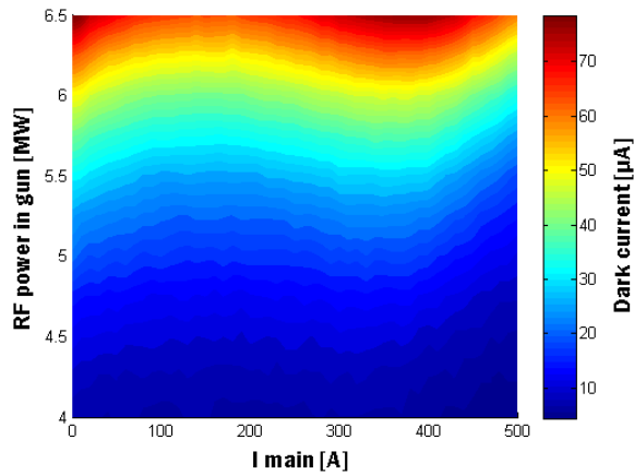
Figure 11: Dark current measurements at different peak power level in the gun vs. main solenoid current.
