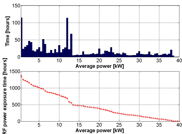
Figure 4: Gun 4.3 run statistics for average power in the gun cavity.
