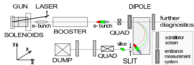
Figure 1: Setup for slice emittance measurements at PITZ
