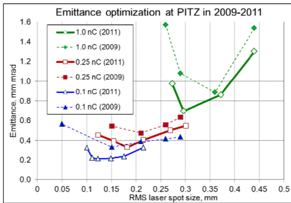
Figure 3: Measured geometric mean emittance as a function of the rms laser spot size for various bunch charges. Results of 2009 are shown with dashed lines.
