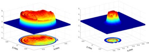
Figure 2: Laser transverse distribution at the photo cathode: obtained using a BSA diameter of 1.2 mm (left plot, rms sizes are \sigma_x=0.30 mm and \sigma_y=0.29 mm) and of 0.5 mm (right plot, \sigma_x=0.13 mm, \sigma_y=0.12 mm).
