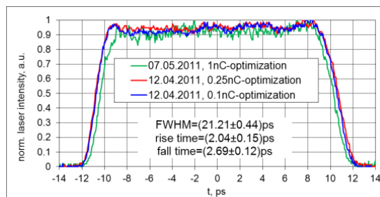
Figure 1: Temporal profiles of a photo cathode laser pulse. Each profile corresponds to the measured emittance optimum for a given bunch charge.
