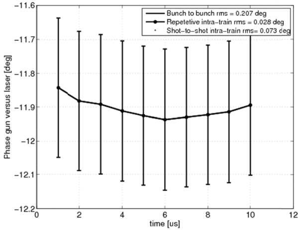
Figure 5: Phase stability along macro pulse.
