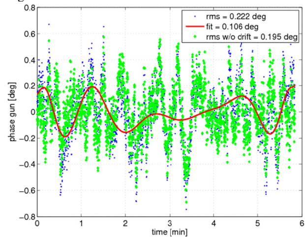
Figure 3: Phase stability measurement by on-line monitoring tool.
