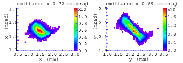
Figure 5: Measured horizontal (left) and vertical (right) phase-space distributions for a bunch charge of 1 nC.
