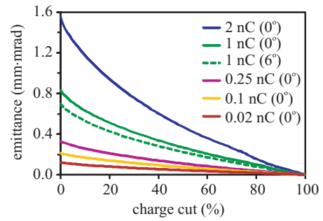
Figure 9: Geometric mean emittance ( \epsilon_{xy} ) as a function of charge cut for different bunch charges.
