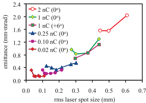
Figure 7: Measured geometric mean emittance ( \epsilon_{xy} ) as a function of the rms laser spot size for different bunch charges. All emittance values were analyzed from the 100% rms phase-space distribution.
