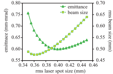
Figure 6: Simulated dependence of emittance and beam size at EMSY1 on the rms laser spot size for a bunch charge of 1 nC. The optimum rms laser spot size of 0.40 mm delivers the minimum emittance of 0.60 mm-mrad.
