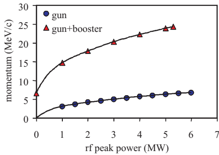
Figure 1: Measured beam mean momentum as a function of the RF power after acceleration with the gun (gun) and the booster (gun+booster). The RF peak power in the gun was set to the maximum value for the momentum measurements after the booster acceleration.
