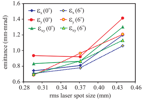
Figure 2: Measured emittance as a function of the rms laser spot size at the cathode for a bunch charge of 1 nC. The gun RF phases of 0^\circ and 6^\circ w.r.t the MMMG phase were used.
