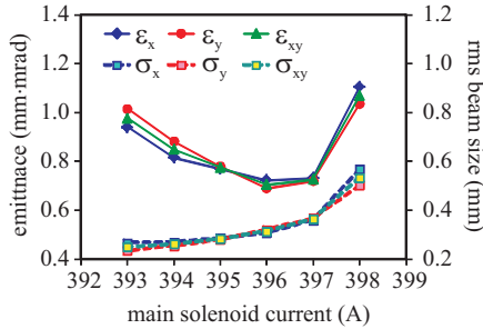
Figure 3: Measured emittance ( \varepsilon ) and rms beam size ( \sigma ) as a function of the main solenoid current for a bunch charge of 1 nC. The gun phase was at 6^\circ from the MMMG phase. The rms laser spot size at the cathode was 0.3 mm.
