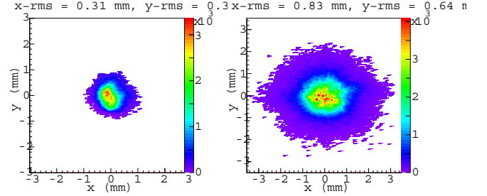
Figure 4: Transverse beam distribution on the YAG screens at EMSY1 (left) and at the beamlet observation station (right) for a bunch charge of 1 nC. The screens are located at 5.74 and 8.38 m downstream of the cathode, respectively.
