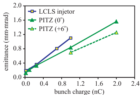
Figure 8: Comparison of measured geometric mean emittance ( \epsilon_{xy} ) as a function of the bunch charge for PITZ and LCLS injector beams.
