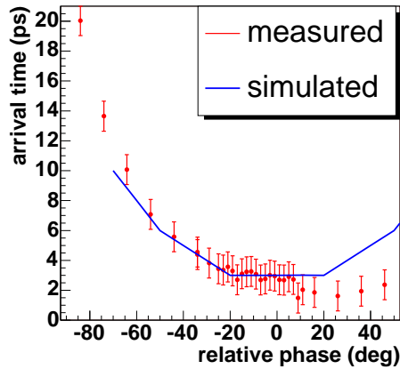
Figure 8: Relative arrival time of the photon pulse produced by the electron bunch at the streak camera as a function of the booster phase. This is assumed to be equal with arrival time of the electron bunch at the screen station
