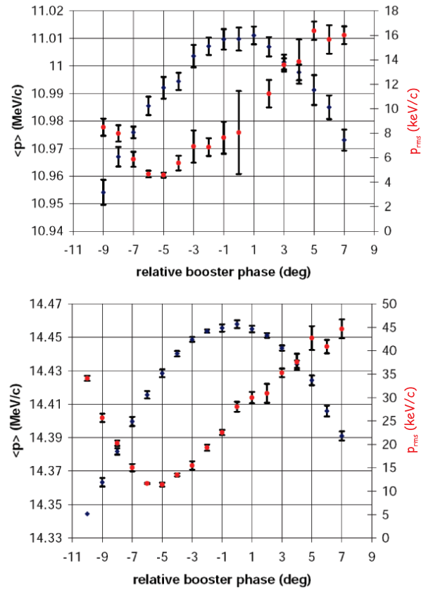
Figure 3: Mean momentum and momentum spread as a function of the booster phase for about 0.6 (top) and 1.9 MW (bottom) in the booster.
