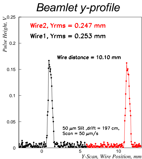
Figure 7: Scan of the beamlet from a 50 \mu\text{m} slit
