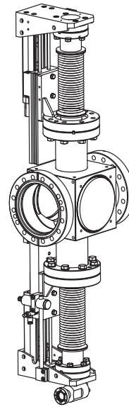
Figure 4: Simplified technical drawing of the screen station.
