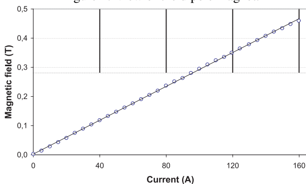
Figure 3: Magnetic field measurements versus applied current.
