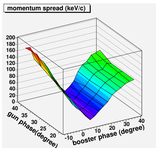
Figure 4: Momentum spread after the booster measured for different booster phases and gun phases.
