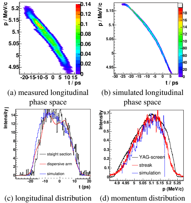
Figure 7: Measured (a) and simulated (b) longitudinal phase space and their projections: longitudinal (c) and momentum (d) distribution for 1.1 nC bunch charge, phase with maximum energy gain +10^\circ and a longitudinal laser distribution with about 20 ps FWHM pulse length. In (c) and (d) the black curves are direct measurements, the red ones are the projections of the measured longitudinal phase space and the blue ones are ASTRA simulations.
