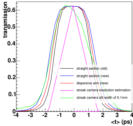
Figure 6: Effect of the dispersion on the resolution by using an optical transmission filter of 550nm with a bandwidth of 10nm (FWHM) compared with the resolution of the streak camera C5680 [4] and the influence of a 0.1 mm streak camera slit width to the resolution.
