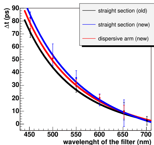
Figure 5: Arrival time of photons with different wavelength.
