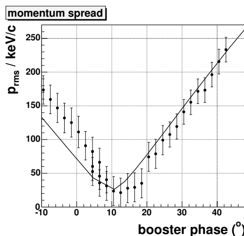
Figure 2: Momentum spread after the booster measured for different booster phases at a gun phase with maximum energy gain. The solid line presents the results from ASTRA simulations.
