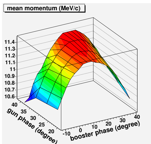
Figure 3: Mean momentum after the booster measured for different booster phases and gun phases.
