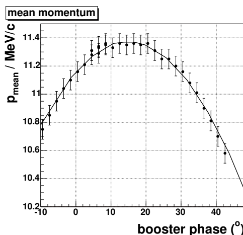
Figure 1: Mean momentum after the booster measured for different booster phases at a gun phase with maximum energy gain. The solid line presents the results from ASTRA simulations.
