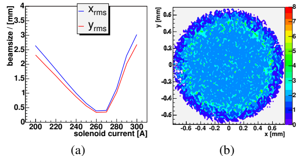
Figure 2: Simulations of the electron beam size as a function of the solenoid current (a) and transverse beam properties at the screen station (b) for a gun and booster phase with maximum energy gain and a flat-top longitudinal laser distribution at 1 nC.
