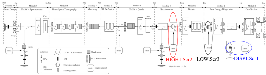
Figure 1: Planed setup of PITZ2. The screen station HIGH1.Scr2, LOW.Scr3 and DISPI.Scr1 are marked.
