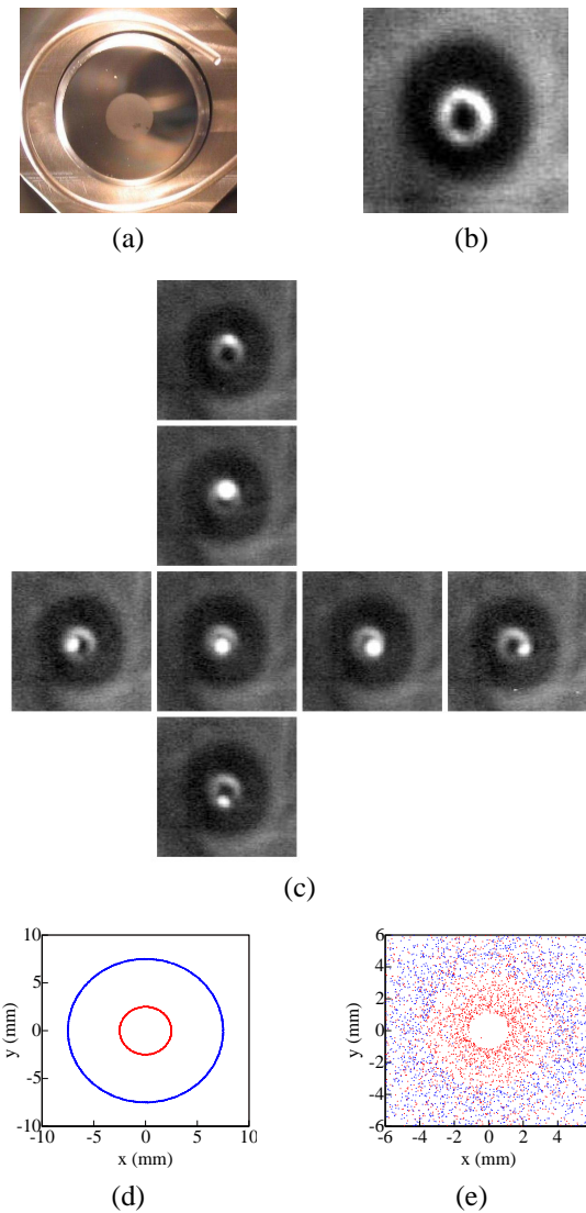
Figure 3: (a) The front surface of the cathode in the cathode chamber. A Cs 2 Te film (2.5 mm radius) is coated on a Mo cathode plug (8 mm radius). The wire surrounding the cathode is an anode used for QE measurement of the cathode. (b) Dark current image at a screen 0.78 m downstream of the cathode. Two ring structures are visible. (c) Electron beam images together with the dark current at the same screen. The emission location of the beam was changed by varying the drive laser location on the cathode by 1 mm steps. Here only every 2 mm step is shown. The measurements have been compared with a numerical simulation with ASTRA [5]. (d) Initial distribution of electrons. (e) Simulation result.
