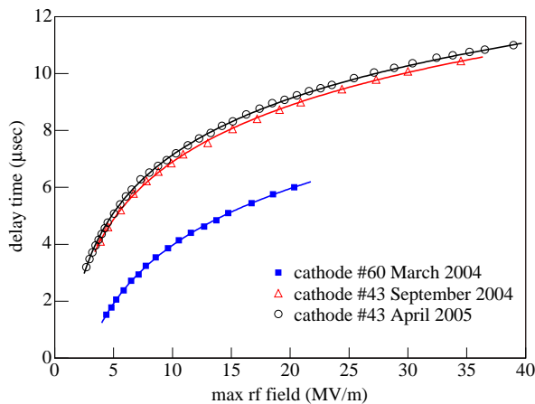
Figure 4: Delay time of the multipacting peak vs. maximum rf field at the cathode. The measurements were made with a main solenoid current of 400 A and a bucking solenoid current of 30 A.
