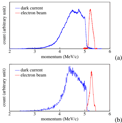
Figure 2: Momentum spectra of dark current and electron beam: (a) measurement with a spectrometer dipole and (b) simulation assuming 47 MV/m maximum field strength at the cathode.
