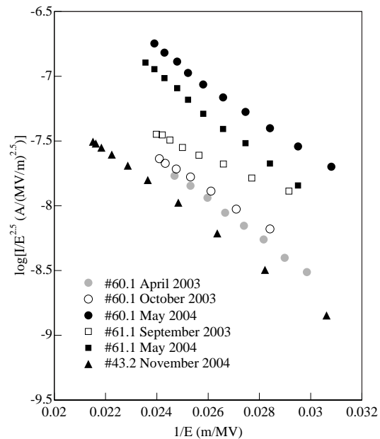
Figure 1: Fowler-Nordheim plots for different status of the cathodes and the cavities. In September 2003 cathode #61.1 [2] was used the very first time. Cavity #2 was used until November 2003 and cavity #1 is being used since January 2004. In May 2004 the Cs 2 Te film of cathode #60.1 was damaged. Cathode #43.2 was very fresh and well conditioned in November 2004.
