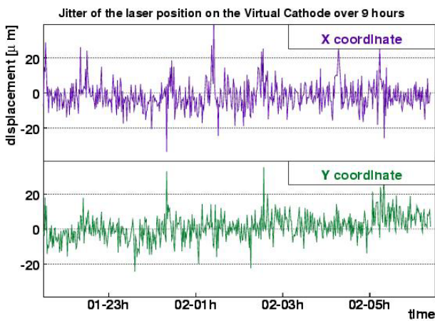
Fig. 5: Jitter of the laser position on VC1 over 9 hours
