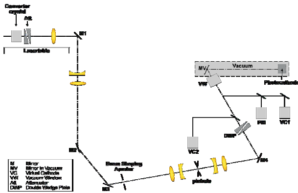
Fig. 2: Schematic of the laser beam-line
