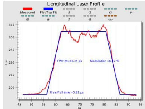
Fig. 6: Longitudinal laser pulse profile
