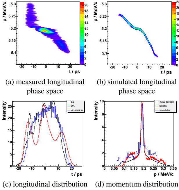
Figure 2: Measured (a) and simulated (b) longitudinal phase space and their projections: longitudinal (c) and momentum (d) distribution for 1 nC bunch charge, optimum launch phase and a flat-top laser distribution with about 20 ps FWHM pulse length. In (c) and (d) the black curves are direct measurements, the red ones are the projections of the measured longitudinal phase space and the blue ones are simulations.
