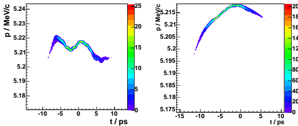
(a) simulated longitudinal phase space 3.45 m downstream from the cathode (b) simulated longitudinal phase space at the exit of the gun
