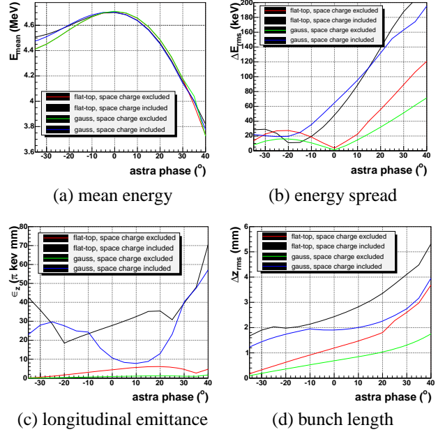
Figure 6: Simulated mean energy (a), energy spread (b), longitudinal emittance (c) and bunch length (d) as a function of the launch phase.
