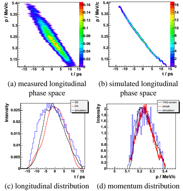
Figure 4: Measured (a) and simulated (b) longitudinal phase space and their projections: longitudinal (c) and momentum distribution (d) for 1 nC bunch charge, optimum launch phase and Gaussian laser distribution with about 10 ps FWHM pulse length. In (c) and (d) the black curves are direct measurements, the red ones are the projections of the measured longitudinal phase space and the blue ones are simulations.
