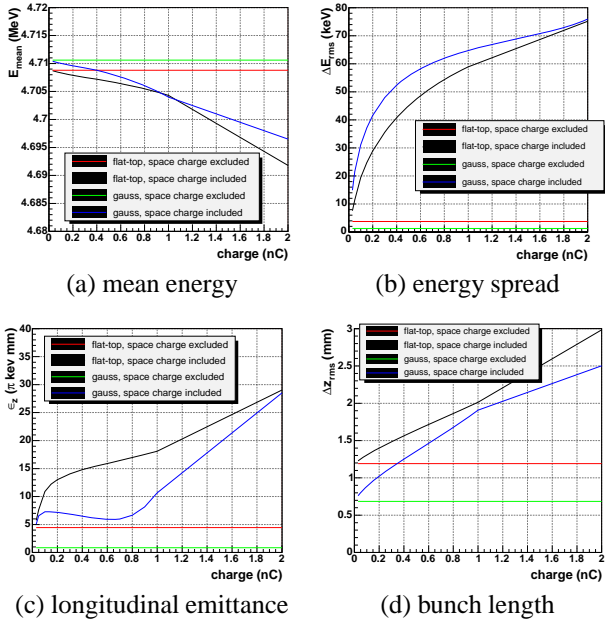
Figure 5: Simulated mean energy (a), energy spread (b), longitudinal emittance (c) and bunch length (d) as a function of the bunch charge.
