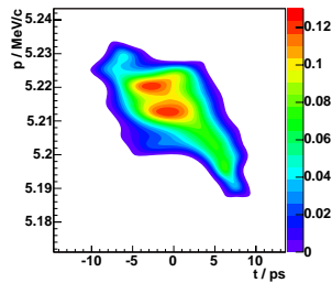
(c) measured longitudinal phase space 3.45 m downstream from the the cathode
