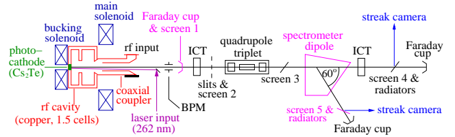
Figure 1: Schematic of PITZ1 setup.
