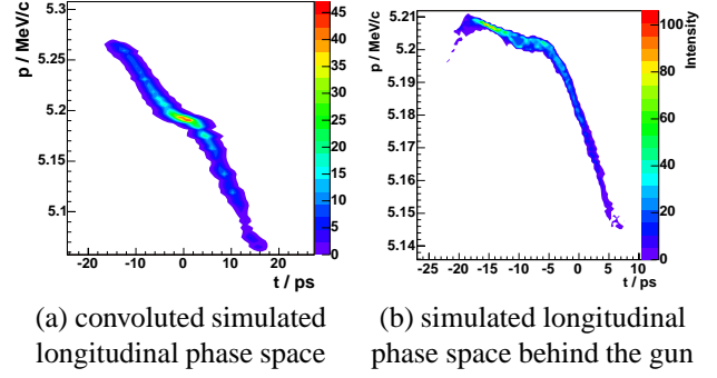
Figure 3: Simulated longitudinal phase space for optimum launch phase, flat-top laser distribution and 1 nC bunch charge (Fig. 2 (b)) convoluted with the resolution function of the streak camera (a). For studying the evolution of the longitudinal phase space the simulated longitudinal phase space for optimum launch phase, flat-top laser distribution and 1 nC bunch charge at the gun exit is shown (b).
