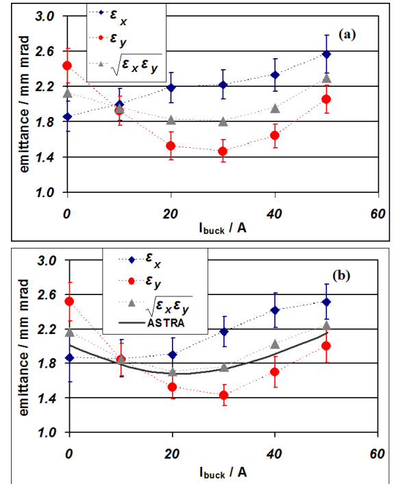
Figure 3: Projected normalized emittance for different bucking solenoid currents. The bunch charge is 1.0 nC, the main solenoid was set to 305 A. The the gun phase is: (a) \phi - \phi_m = 0^\circ , and (b) \phi - \phi_m = -5^\circ . The horizontal and vertical emittance as well as their geometrical average are shown. The solid line in the lower graph represents a corresponding ASTRA simulation at the geometrical average.
