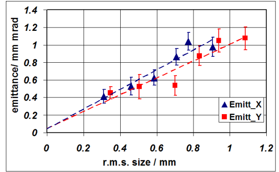
Figure 5: Transverse emittance vs. laser spot r.m.s. size measured with the slit scanning technique at 3 pC.
