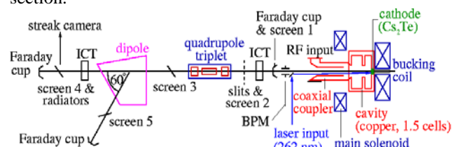
Figure 1: Layout of PITZ.
