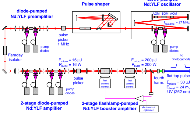
Figure 2: Layout of the PITZ laser system.
