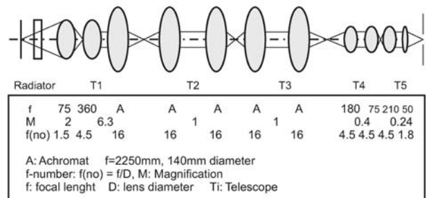
Fig. 5: Scheme of the full optical transmission line
