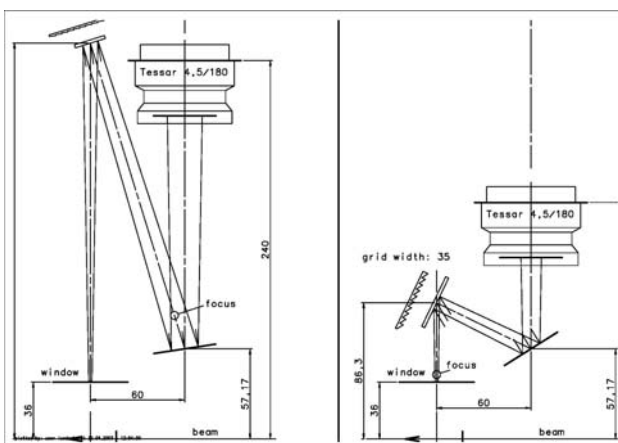
Fig. 3: Scheme using reflection grating
