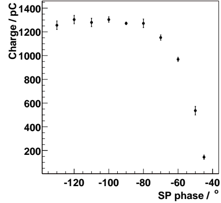
Figure 4: Measured electron bunch charge as a function of set point phase.
