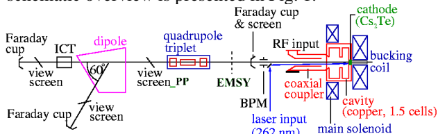
Figure 1: Schematics of the current set-up.
