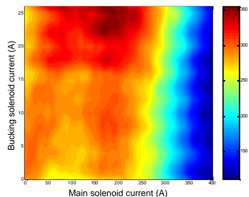
Figure 3: Contour plot of the dark current at 40 MV/m for the \text{Cs}_2\text{Te} cathode as a function of main solenoid and bucking solenoid currents.
