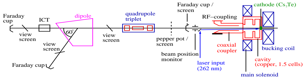
Figure 1: Schematic of the photoinjector.
